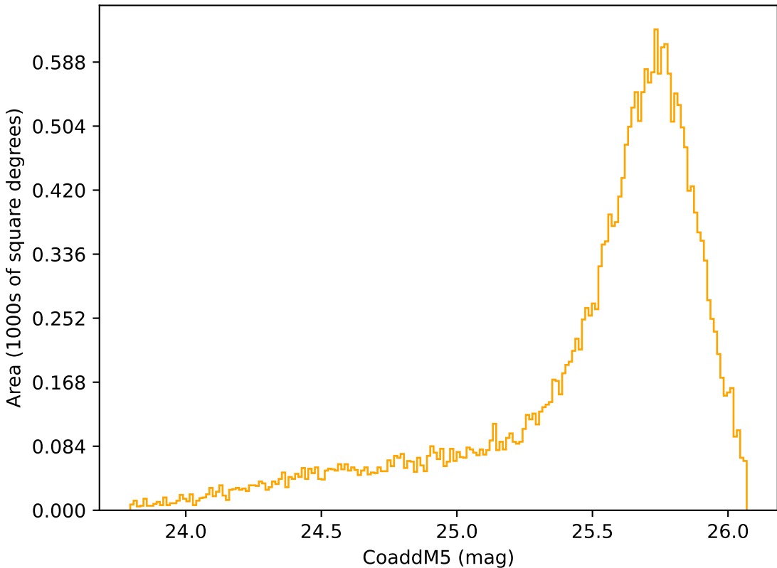
baseline_v3.0_10yrs Yr 1 r band: CoaddM5
