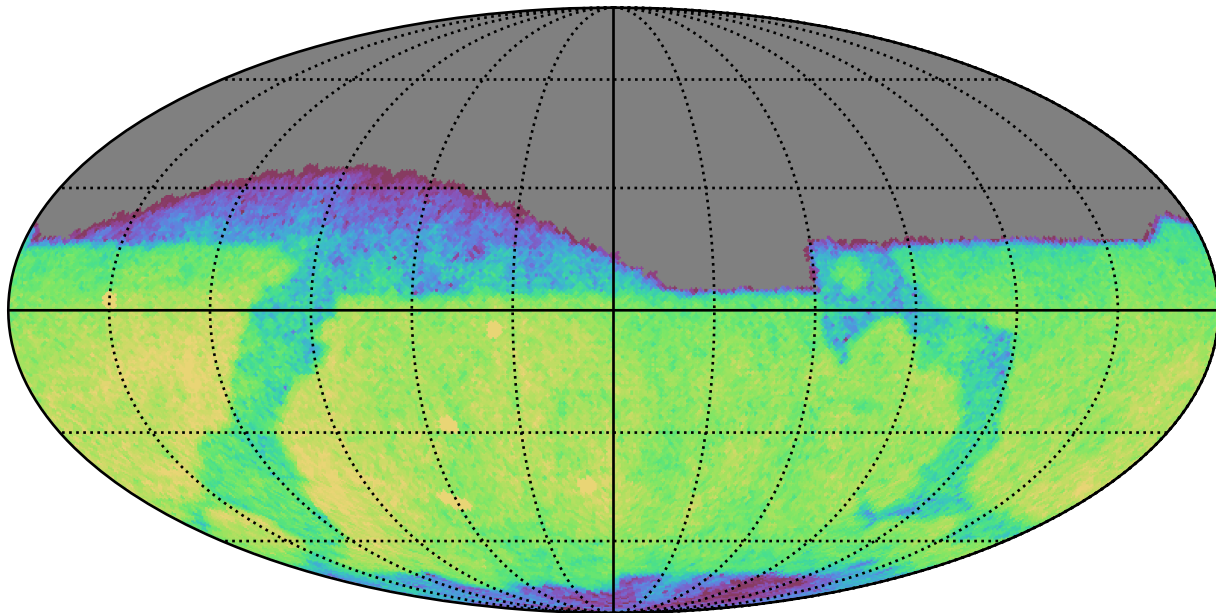
baseline_v3.0_10yrs Yr 1 i band: CoaddM5
