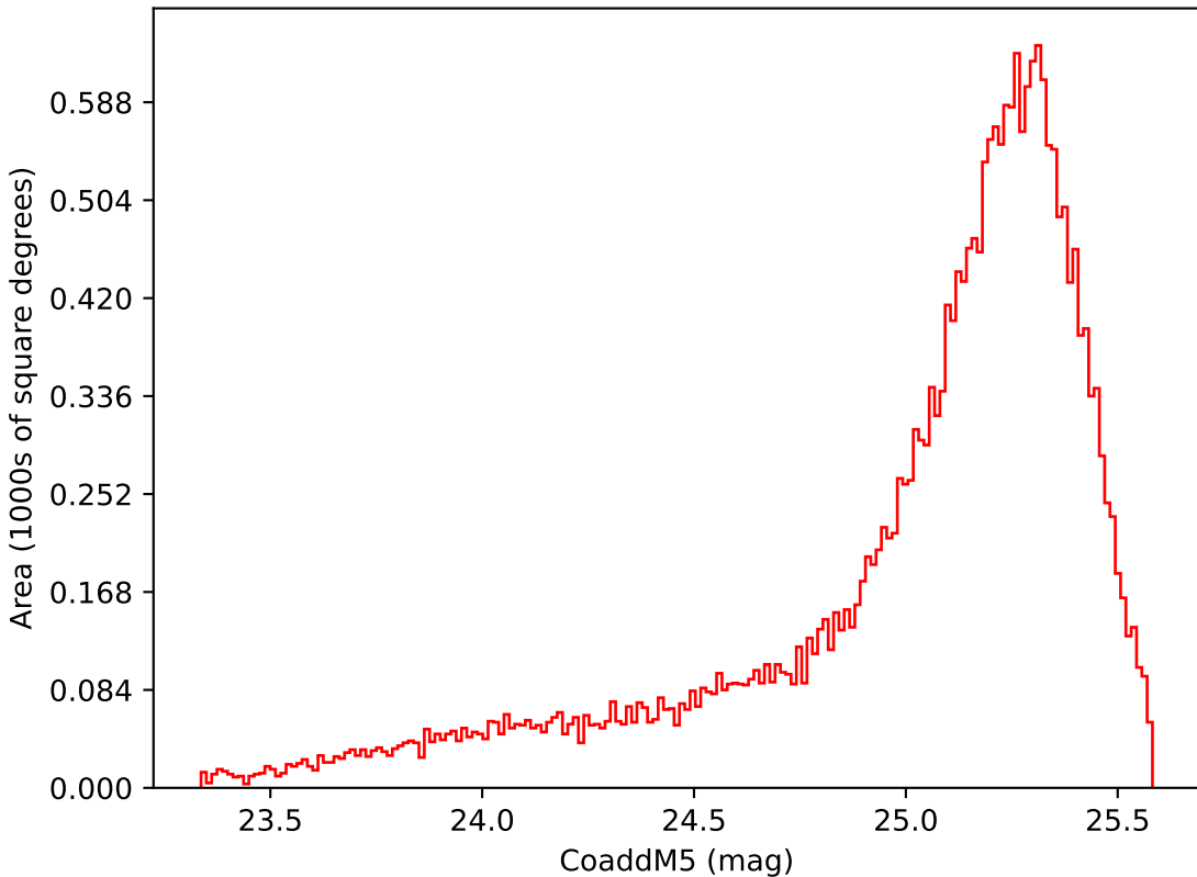
baseline_v3.0_10yrs Yr 1 i band: CoaddM5
