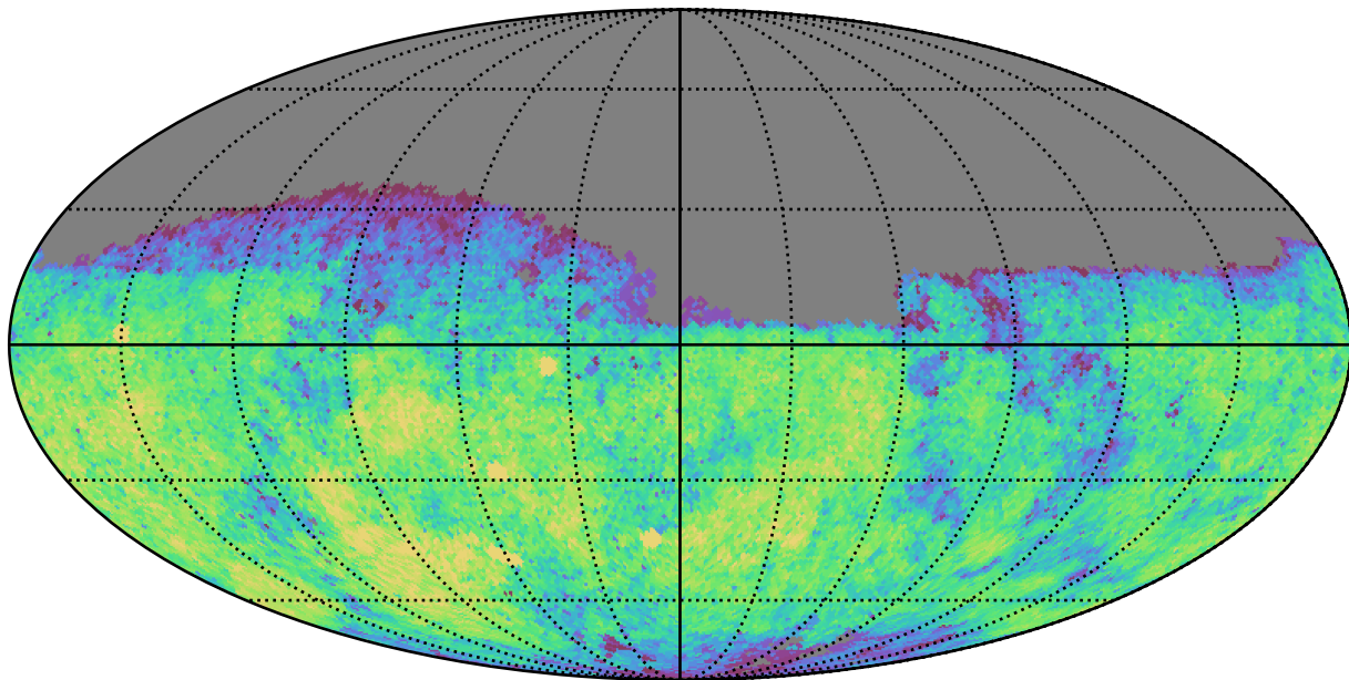
baseline_v3.0_10yrs Yr 1 g band: CoaddM5
