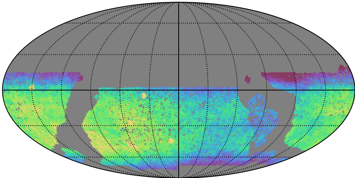
baseline_v3.0_10yrs WFD z band: CoaddM5
