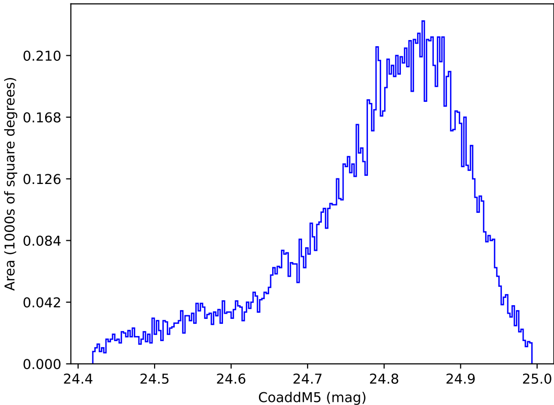
baseline_v3.0_10yrs WFD y band: CoaddM5
