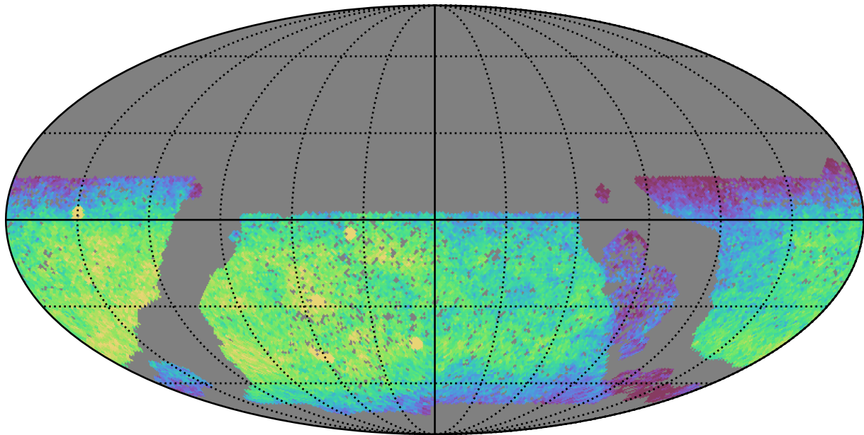
baseline_v3.0_10yrs WFD u band: CoaddM5
