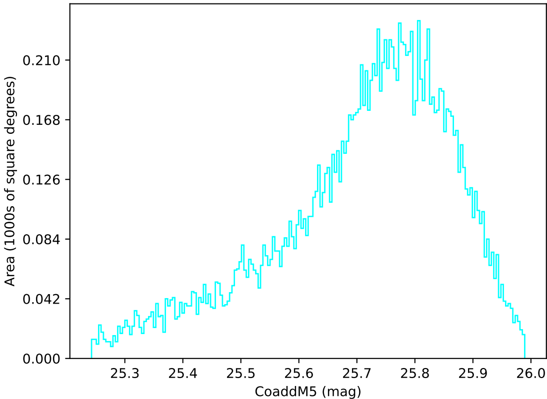
baseline_v3.0_10yrs WFD u band: CoaddM5
