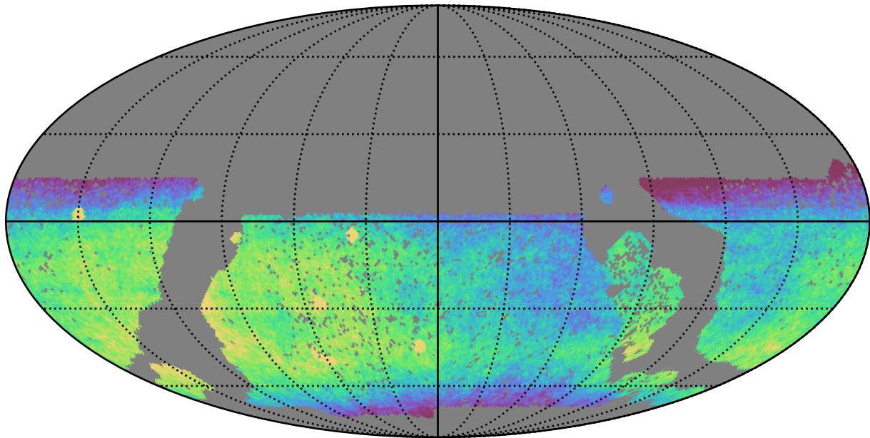
baseline_v3.0_10yrs WFD r band: CoaddM5
