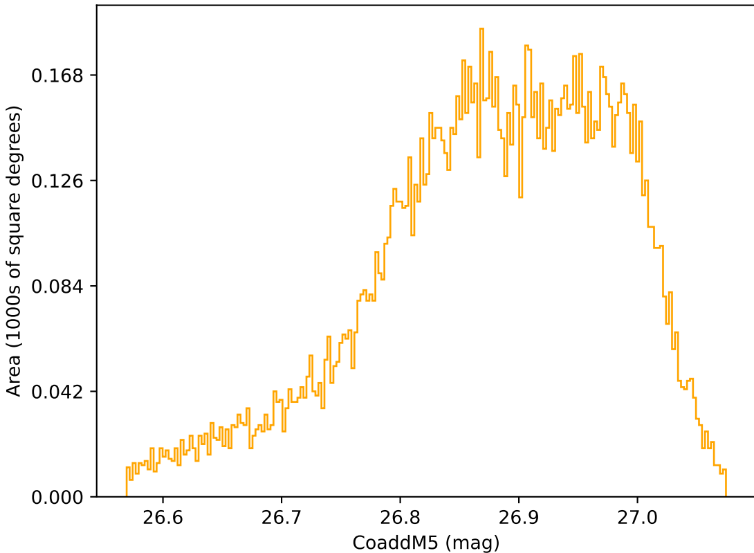
baseline_v3.0_10yrs WFD r band: CoaddM5
