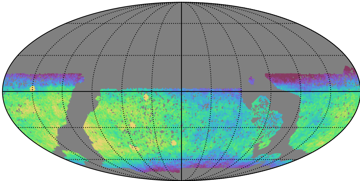
baseline_v3.0_10yrs WFD i band: CoaddM5
