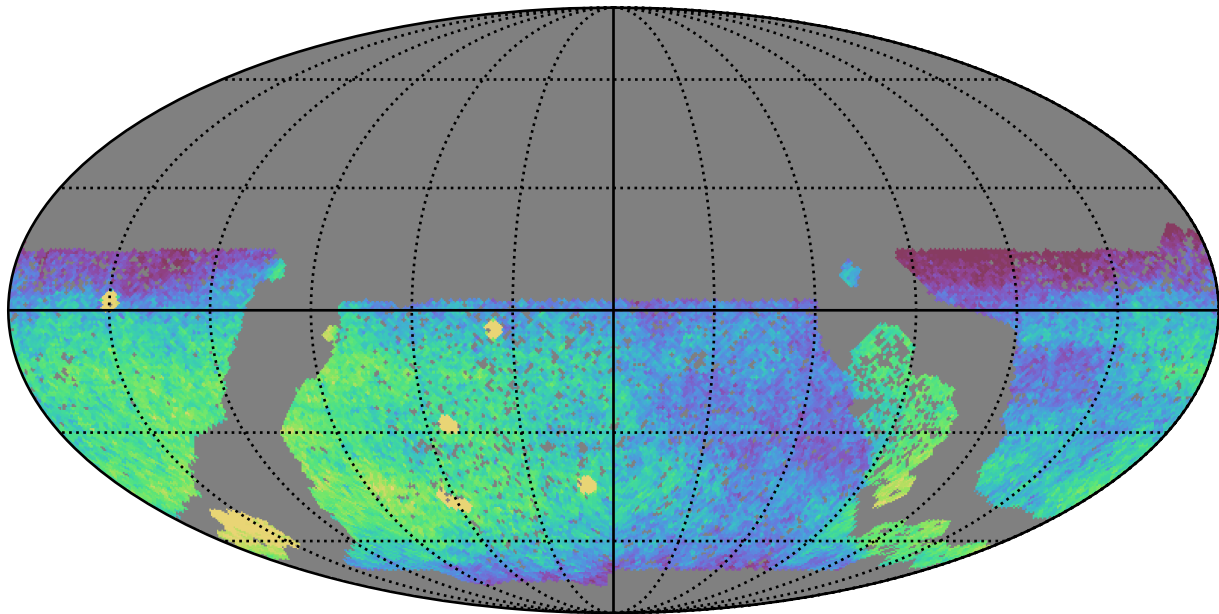
baseline_v3.0_10yrs WFD g band: CoaddM5
