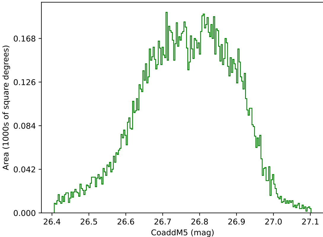
baseline_v3.0_10yrs WFD g band: CoaddM5
