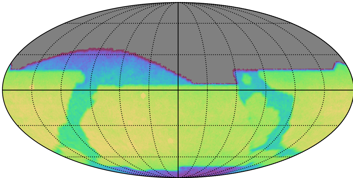
baseline_v3.0_10yrs All sky z band: CoaddM5
