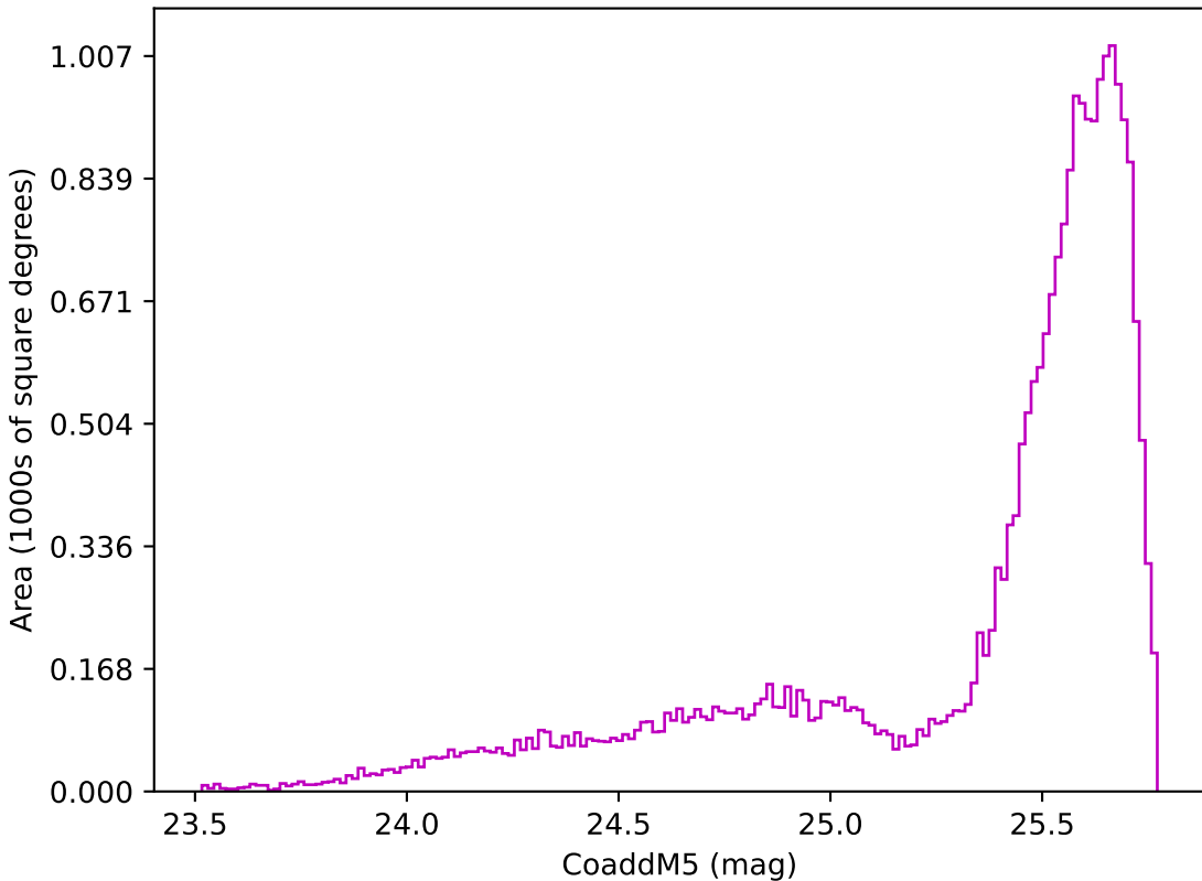
baseline_v3.0_10yrs All sky z band: CoaddM5
