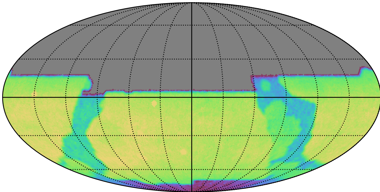
baseline_v3.0_10yrs All sky y band: CoaddM5
