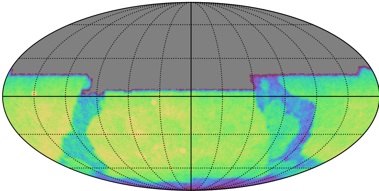
baseline_v3.0_10yrs All sky u band: CoaddM5
