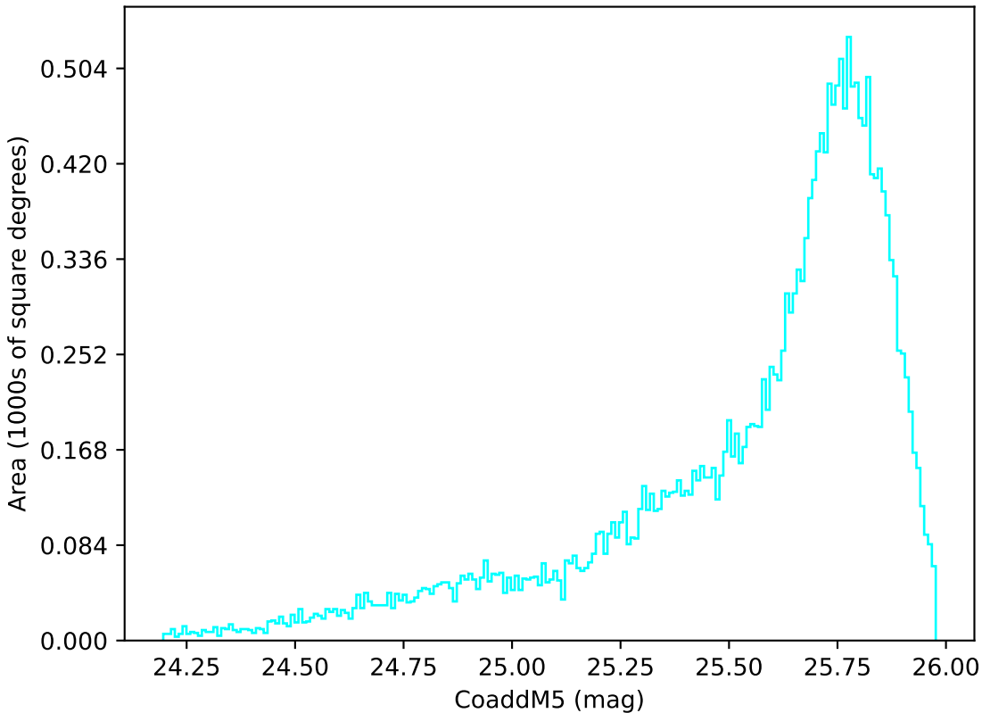
baseline_v3.0_10yrs All sky u band: CoaddM5
