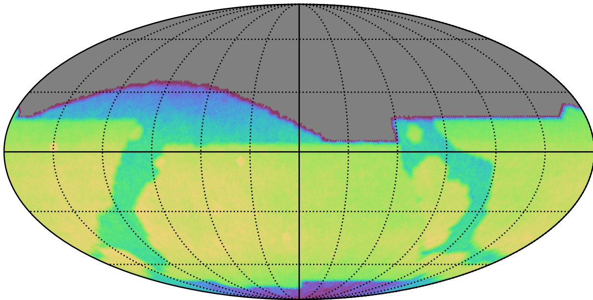
baseline_v3.0_10yrs All sky r band: CoaddM5
