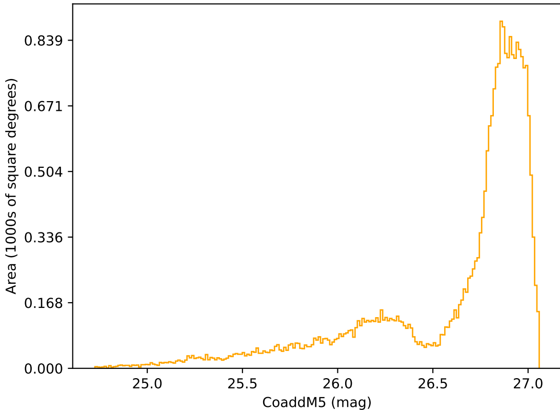
baseline_v3.0_10yrs All sky r band: CoaddM5
