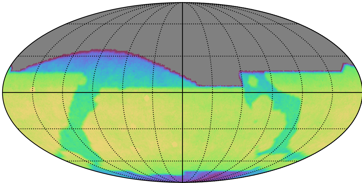
baseline_v3.0_10yrs All sky i band: CoaddM5
