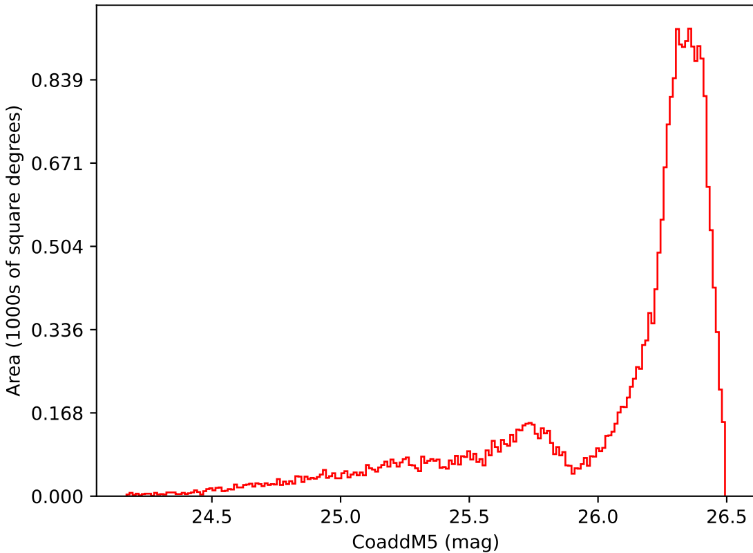
baseline_v3.0_10yrs All sky i band: CoaddM5
