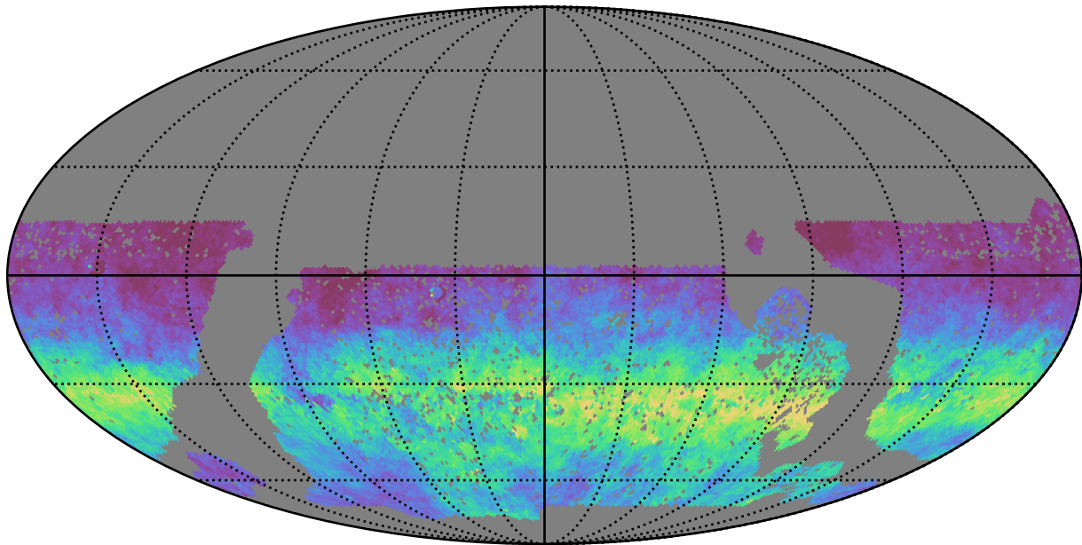
baseline_v3.0_10yrs WFD z band: AngleRms rotSkyPos
