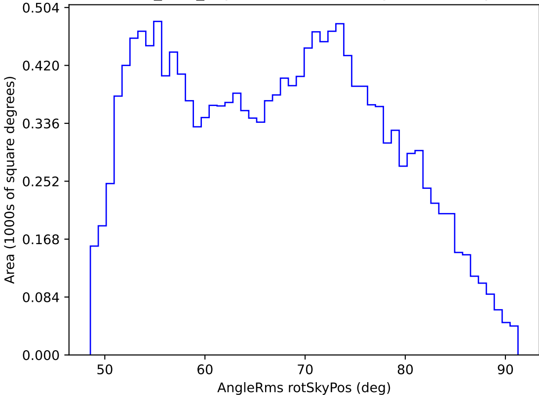
baseline_v3.0_10yrs WFD z band: AngleRms rotSkyPos
