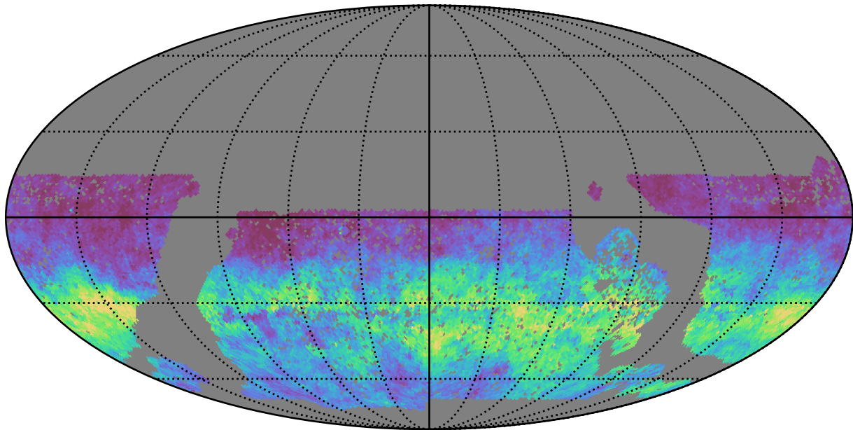
baseline_v3.0_10yrs WFD y band: AngleRms rotSkyPos
