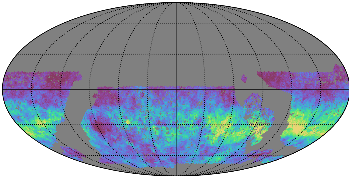
baseline_v3.0_10yrs WFD u band: AngleRms rotSkyPos
