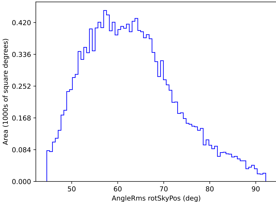
baseline_v3.0_10yrs WFD u band: AngleRms rotSkyPos
