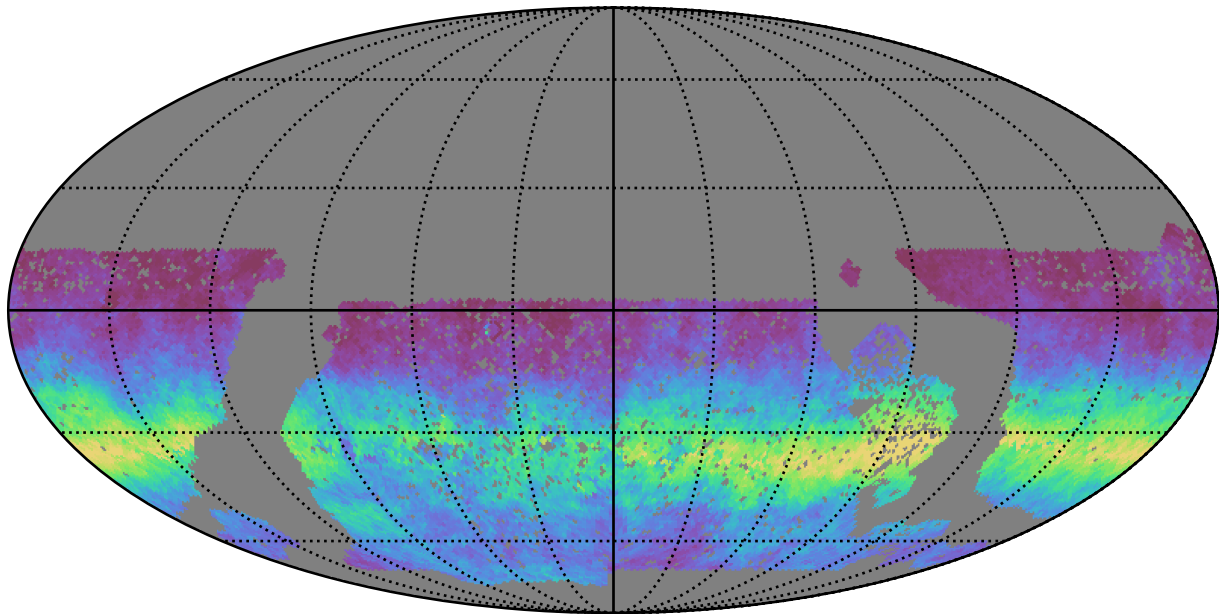
baseline_v3.0_10yrs WFD r band: AngleRms rotSkyPos
