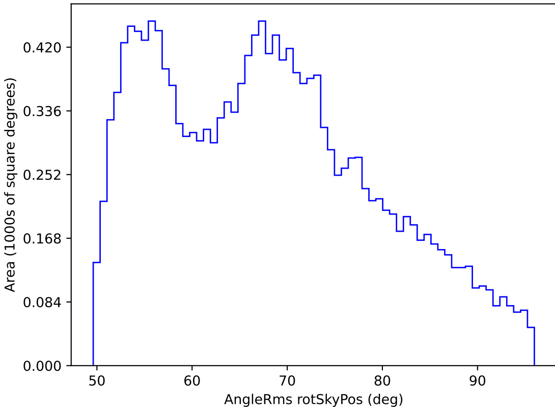
baseline_v3.0_10yrs WFD r band: AngleRms rotSkyPos
