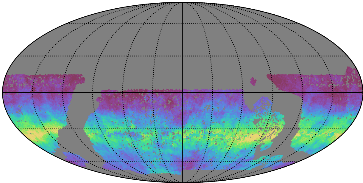
baseline_v3.0_10yrs WFD i band: AngleRms rotSkyPos
