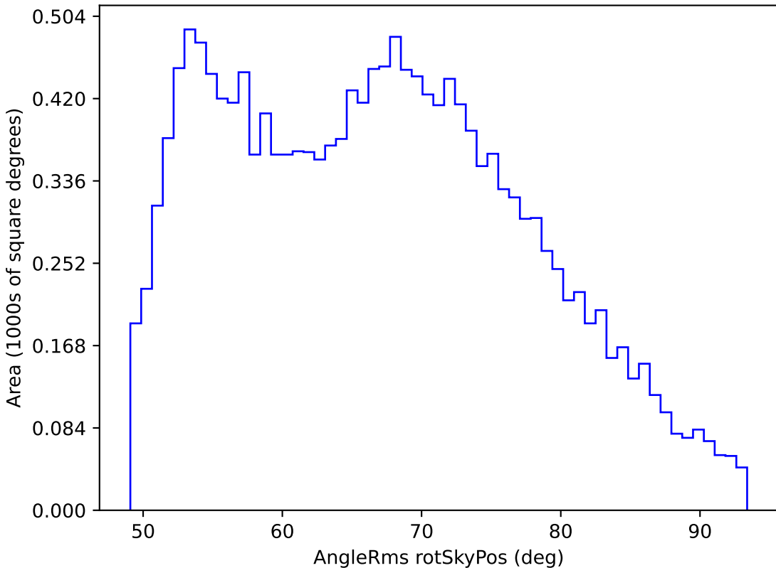
baseline_v3.0_10yrs WFD i band: AngleRms rotSkyPos
