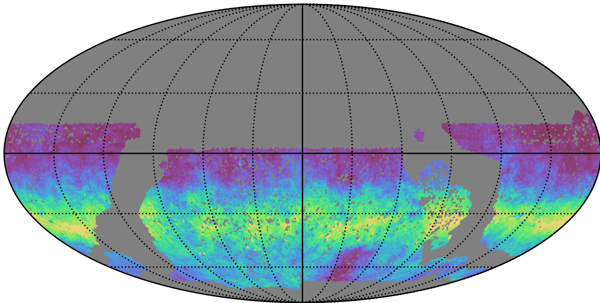
baseline_v3.0_10yrs WFD g band: AngleRms rotSkyPos
