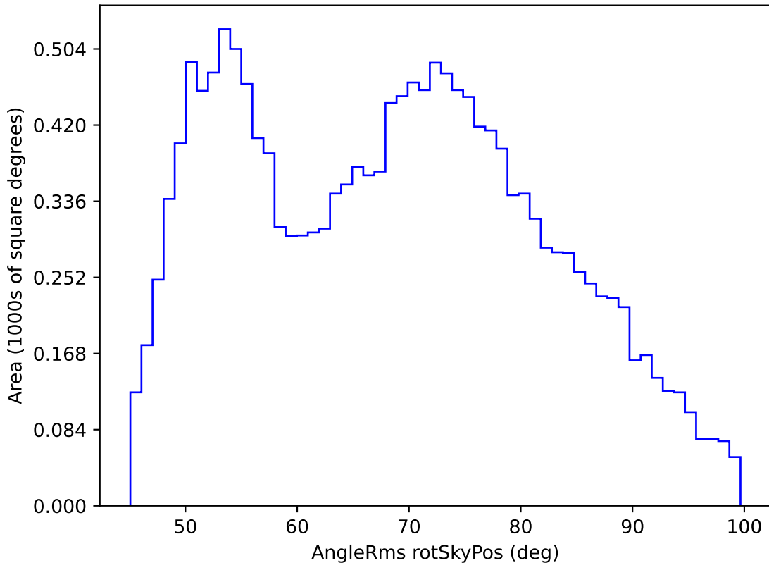
baseline_v3.0_10yrs WFD g band: AngleRms rotSkyPos
