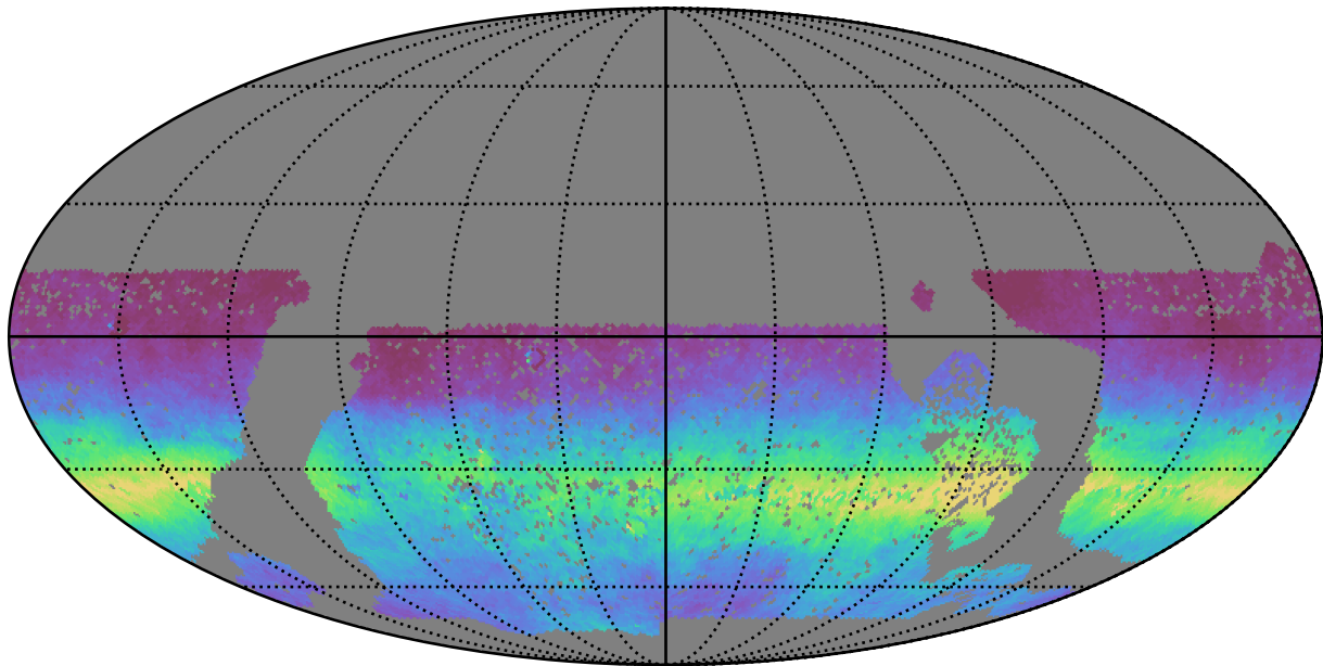
baseline_v3.0_10yrs WFD all bands: AngleRms rotSkyPos
