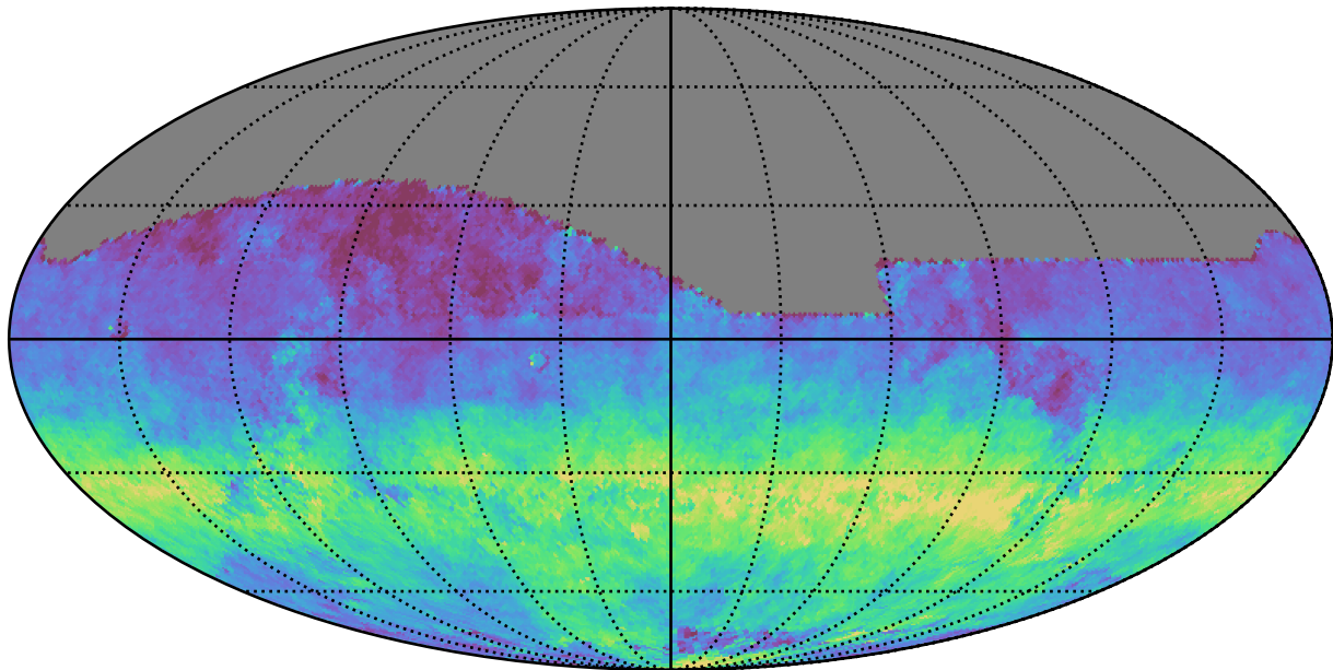
baseline_v3.0_10yrs All sky z band: AngleRms rotSkyPos
