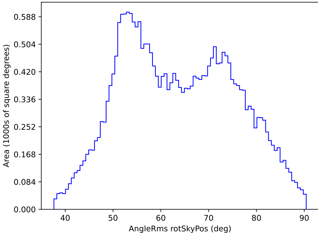
baseline_v3.0_10yrs All sky z band: AngleRms rotSkyPos
