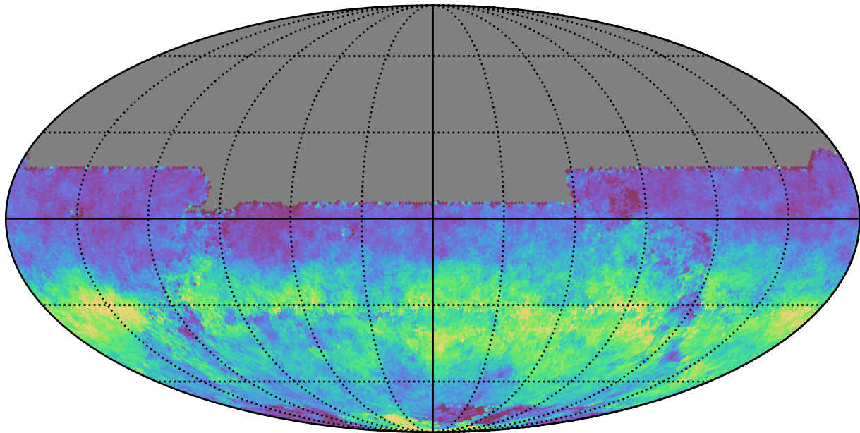
baseline_v3.0_10yrs All sky y band: AngleRms rotSkyPos
