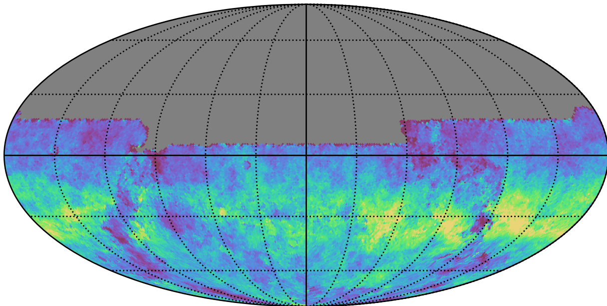
baseline_v3.0_10yrs All sky u band: AngleRms rotSkyPos
