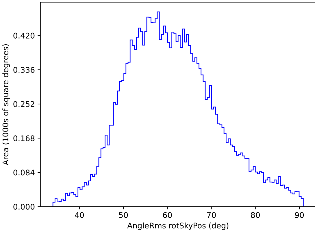
baseline_v3.0_10yrs All sky u band: AngleRms rotSkyPos
