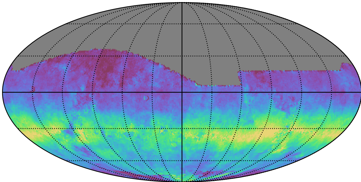
baseline_v3.0_10yrs All sky r band: AngleRms rotSkyPos
