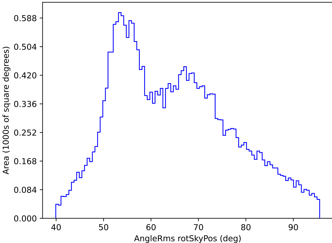
baseline_v3.0_10yrs All sky r band: AngleRms rotSkyPos
