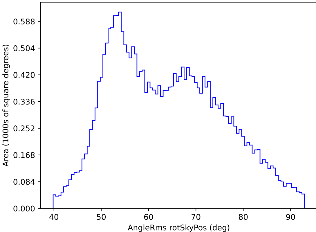
baseline_v3.0_10yrs All sky i band: AngleRms rotSkyPos
