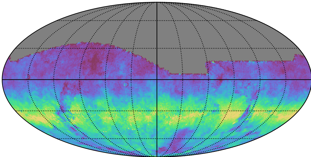
baseline_v3.0_10yrs All sky g band: AngleRms rotSkyPos
