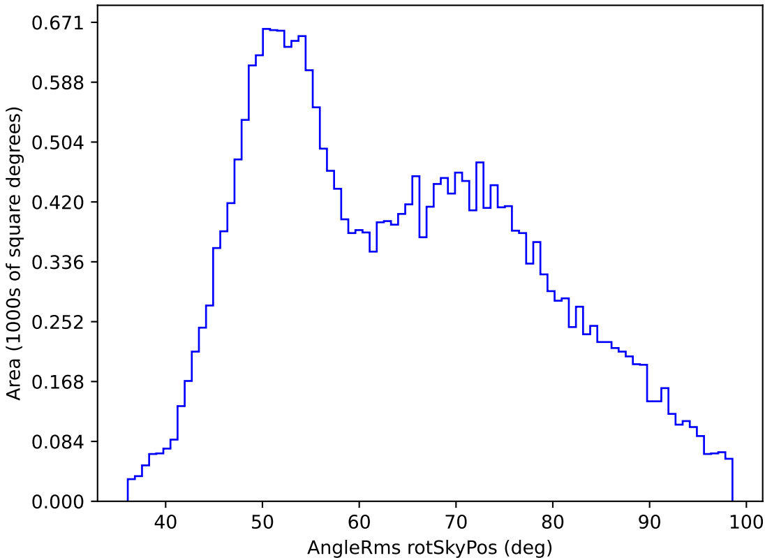
baseline_v3.0_10yrs All sky g band: AngleRms rotSkyPos
