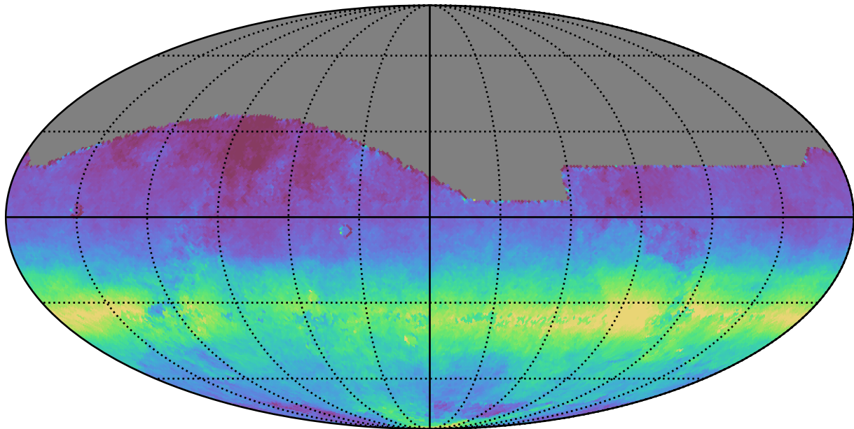
baseline_v3.0_10yrs All sky all bands: AngleRms rotSkyPos
