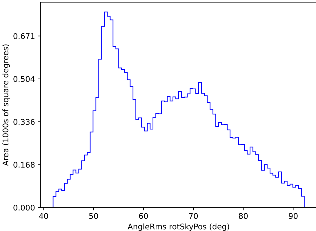
baseline_v3.0_10yrs All sky all bands: AngleRms rotSkyPos
