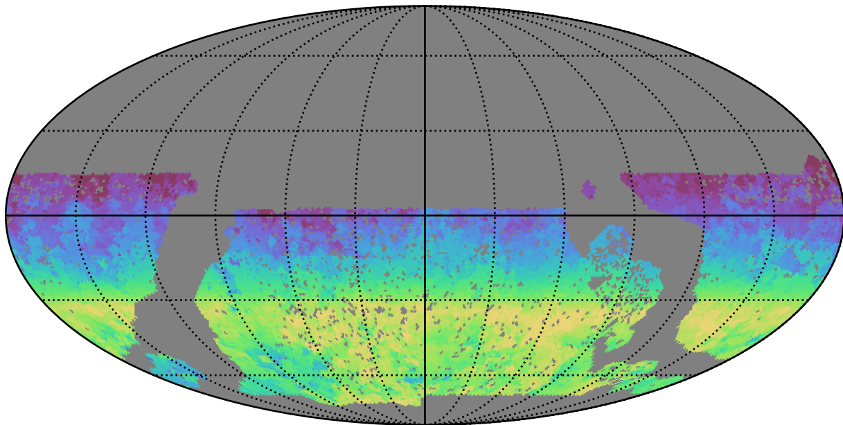
baseline_v3.0_10yrs WFD z band: AngleRange rotSkyPos
