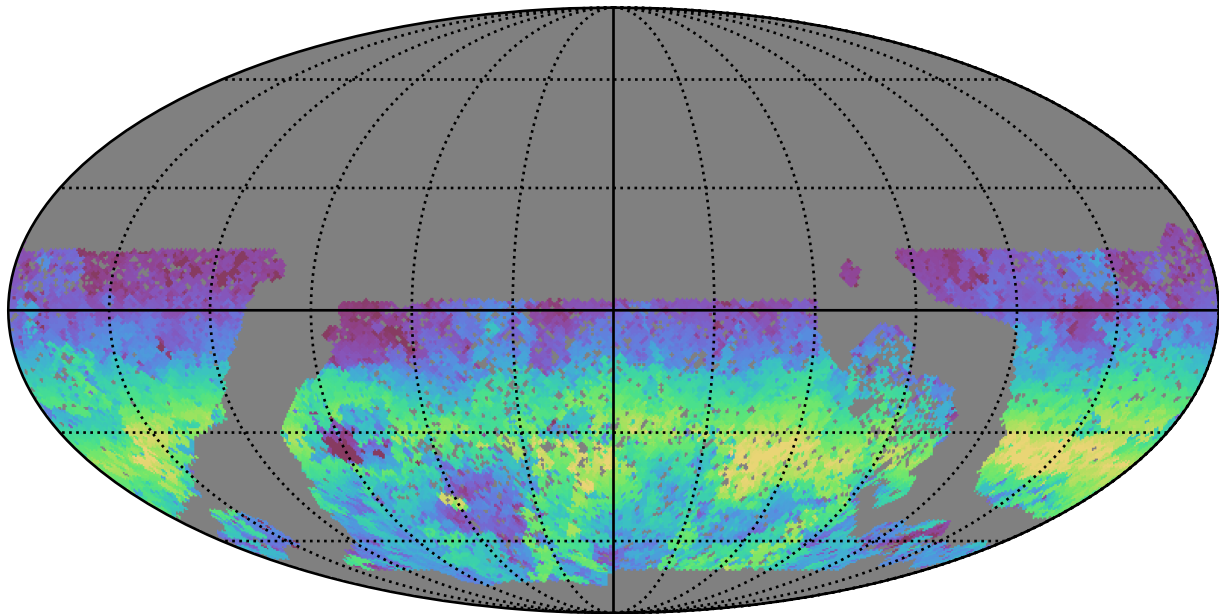
baseline_v3.0_10yrs WFD u band: AngleRange rotSkyPos
