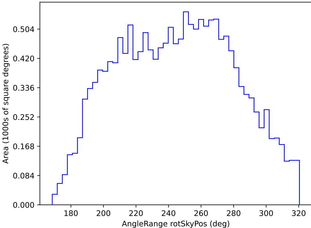
baseline_v3.0_10yrs WFD u band: AngleRange rotSkyPos
