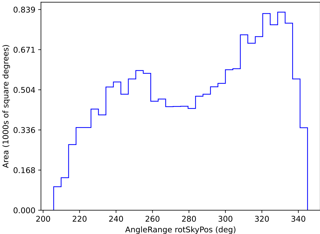
baseline_v3.0_10yrs WFD r band: AngleRange rotSkyPos
